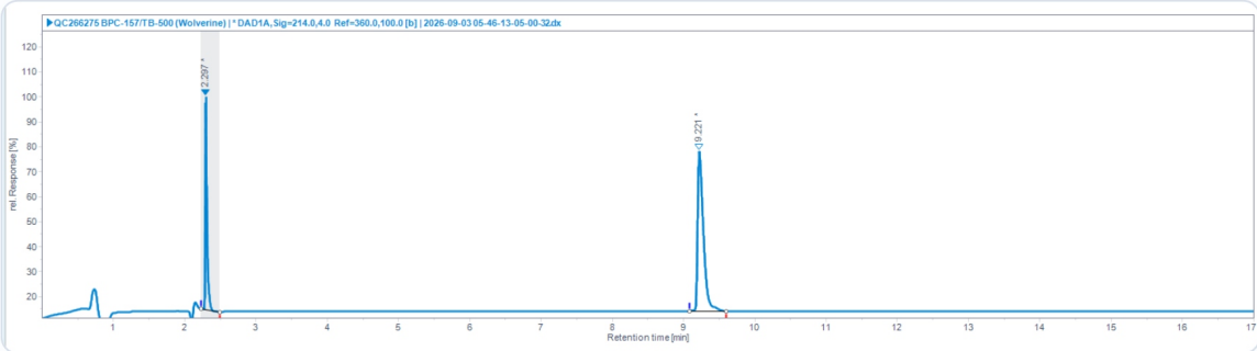
HPLC Chromatogram · Retention Time 2.297, 9.221 min
