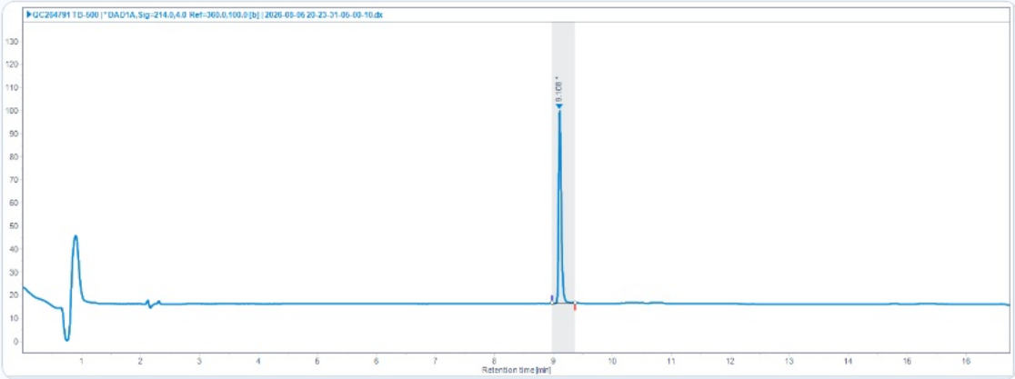
HPLC Chromatogram (Retention Time: 9.108 min)
