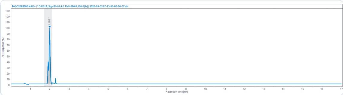
HPLC Chromatogram · Retention Time 1.985 min
